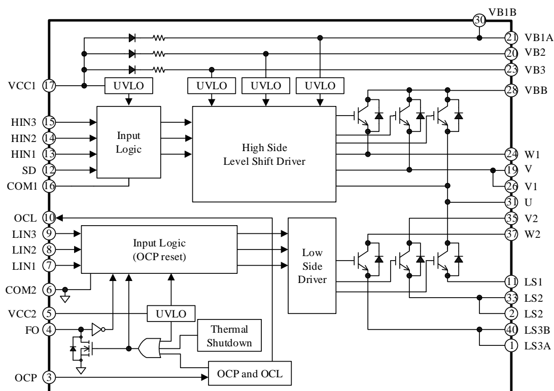
Figure 7-2. SIM6822MV, SIM6827MV, or SIM6880M
