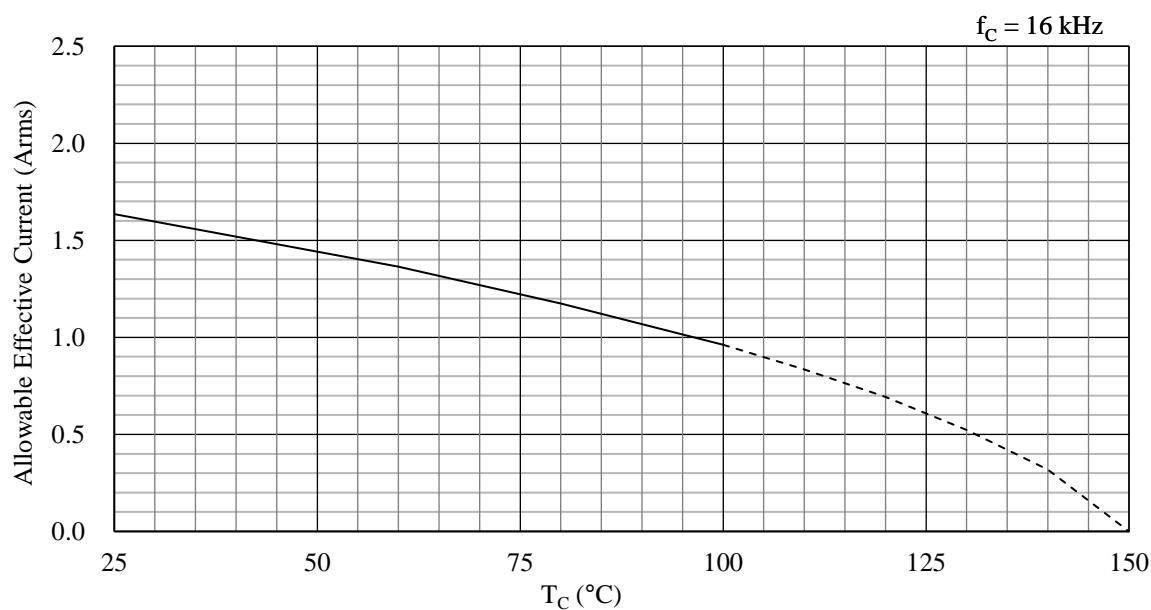
Figure 15-50. Allowable Effective Current ( f_C = 16 \text{ kHz} ): SIM6812M
