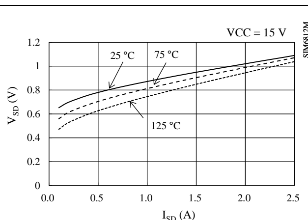
Figure 15-32. Power MOSFET V_{SD} vs. I_{SD}
