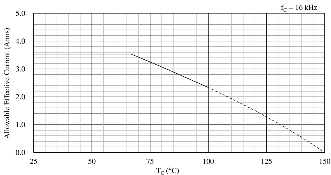
Figure 15-54. Allowable Effective Current ( f_C = 16 kHz): SIM6822MV
