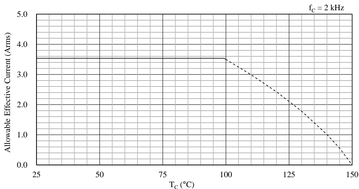
Figure 15-53. Allowable Effective Current ( f_C = 2 kHz): SIM6822MV
