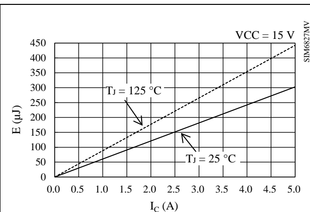
Figure 15-46. Low-side Switching Loss
