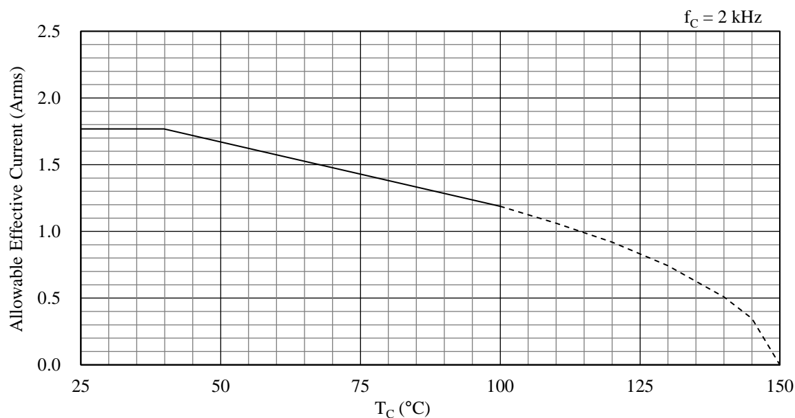
Figure 15-49. Allowable Effective Current ( f_C = 2 \text{ kHz} ): SIM6812M
