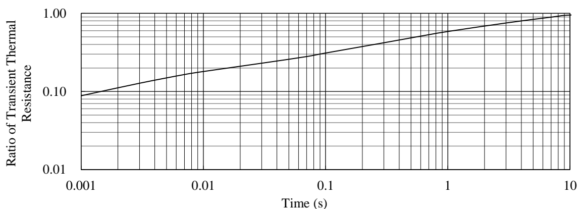
Figure 15-2. Transient Thermal Resistance: SIM6822MV, SIM6827MV
