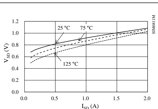
Figure 15-30. Power MOSFET V_{SD} vs. I_{SD}
